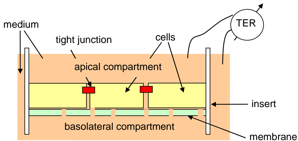
Fig. 9 Polyester filters and cell culture monolayer fully separating the apical and basolateral compartments. Diffusion between these two compartments is only possible via transcellular or paracellular transport.
